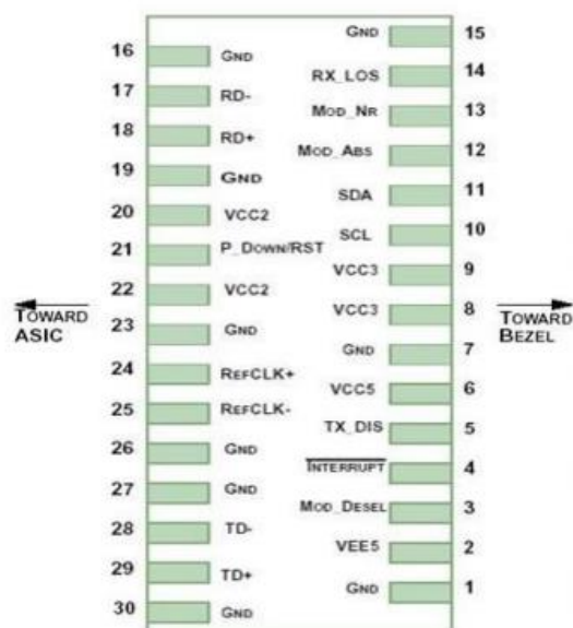
Figure1.Electrical Pin-out Details
