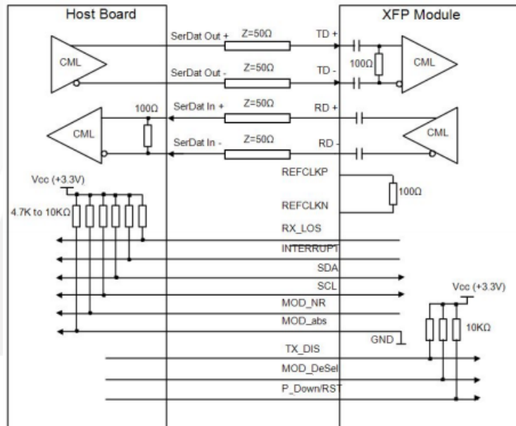
Figure4. Recommended High-speed Interface Circuit
