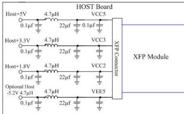
Figure3. Recommended Host Board Power Supply Circuit
